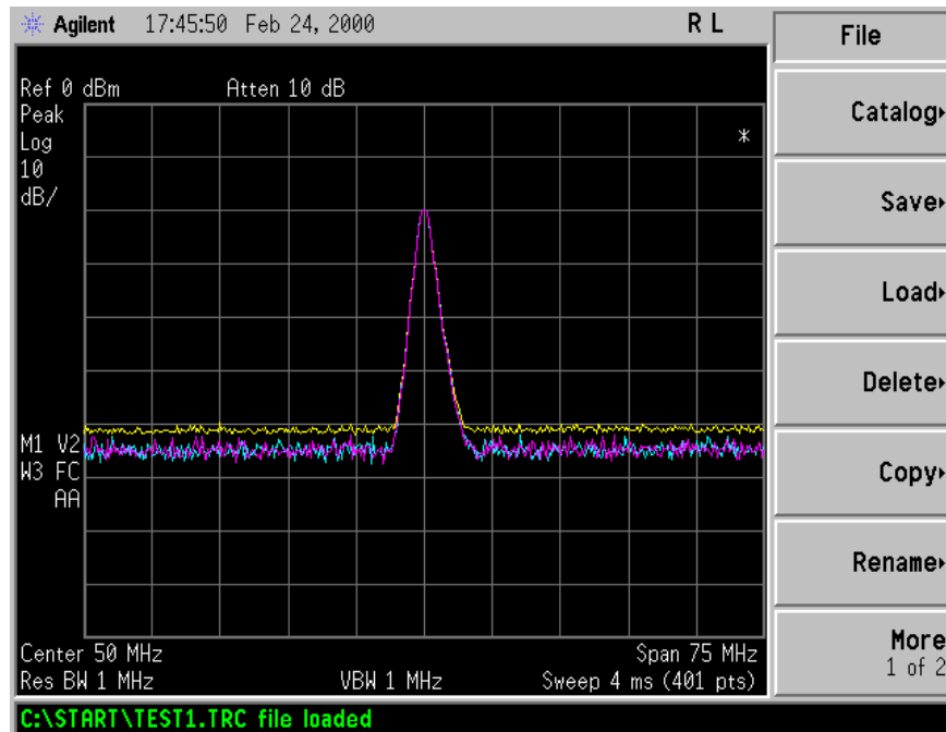
Figure 4-6. File Loaded
